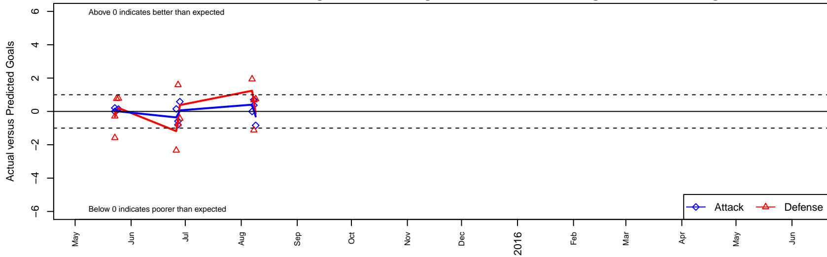
BSC Portland Vapor B00 Dots are actual minus expected GF (blue circles) and GA (red triangles). Blue line is smoothed change in attack strength. Red is smoothed change in defense strength.
